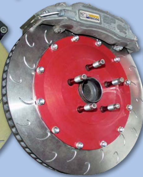
Superlite Calipers
